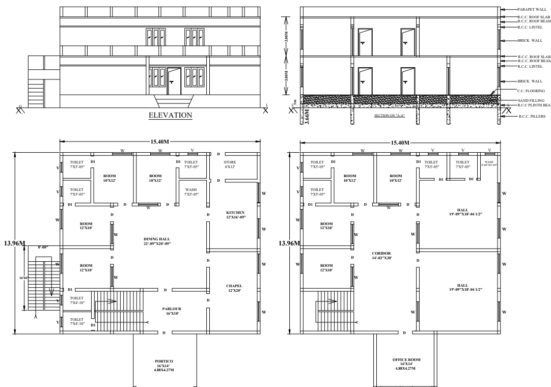
PLAN SHOWING THE PROPOSED CONSTRUCTION OF R.C.C ROOF OF ST. PAUL TAILORING CENTER FOR GIRLS AND UNEMPLOYED WOMEN, GROUND & FIRST FLOOR BUILDING AT PATHARLAPADU VILLAGE, THIRUMALAYAPALEM MANDAL, KHAMMAM DISTRICT, TELANGANA STATE.
